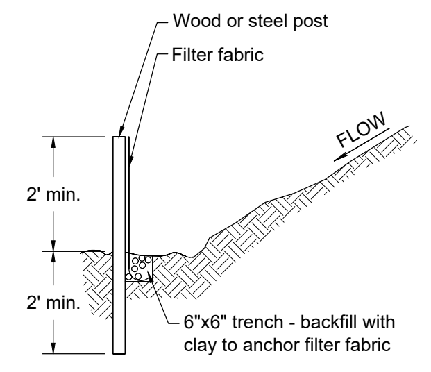
SILT FENCE DETAIL REFER TO METRO DETAIL TCP-13 N.T.S.
