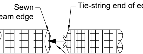
BUTT JOINT DETAIL E1-B1
