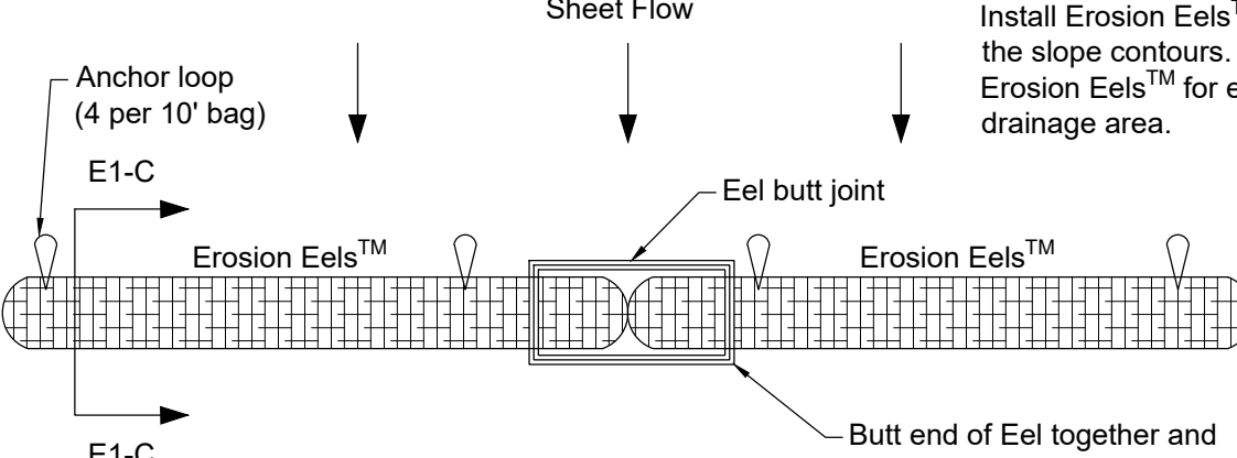
BUTT JOINT DETAIL E1-B1
