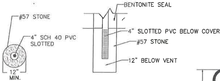
GAS VENT SECTION VIEWS NOT TO SCALE
