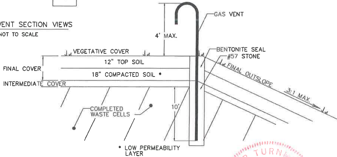
GAS VENT DETAIL
