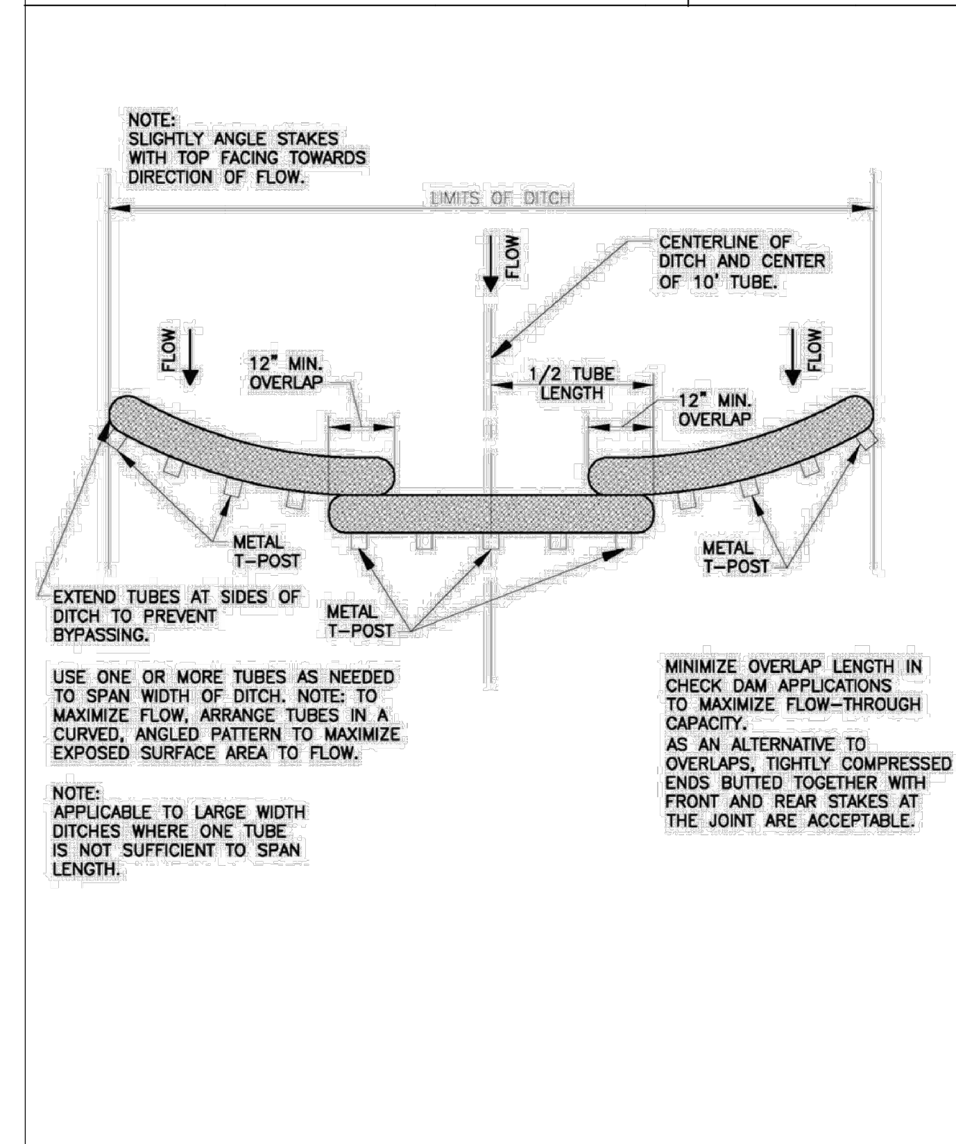
Figure TCP-14-2 Check Dam Arrangement for Larger Width Ditches for Sediment Tubes
