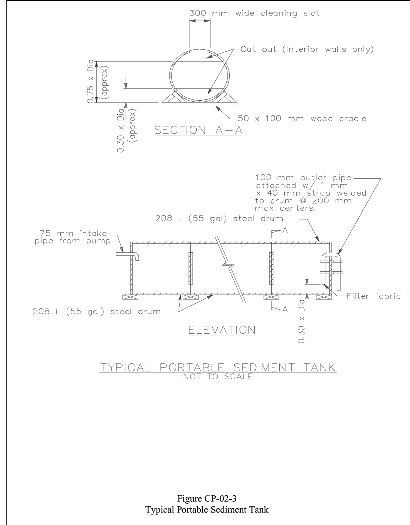
Figure CP-02-3 Typical Portable Sediment Tank
