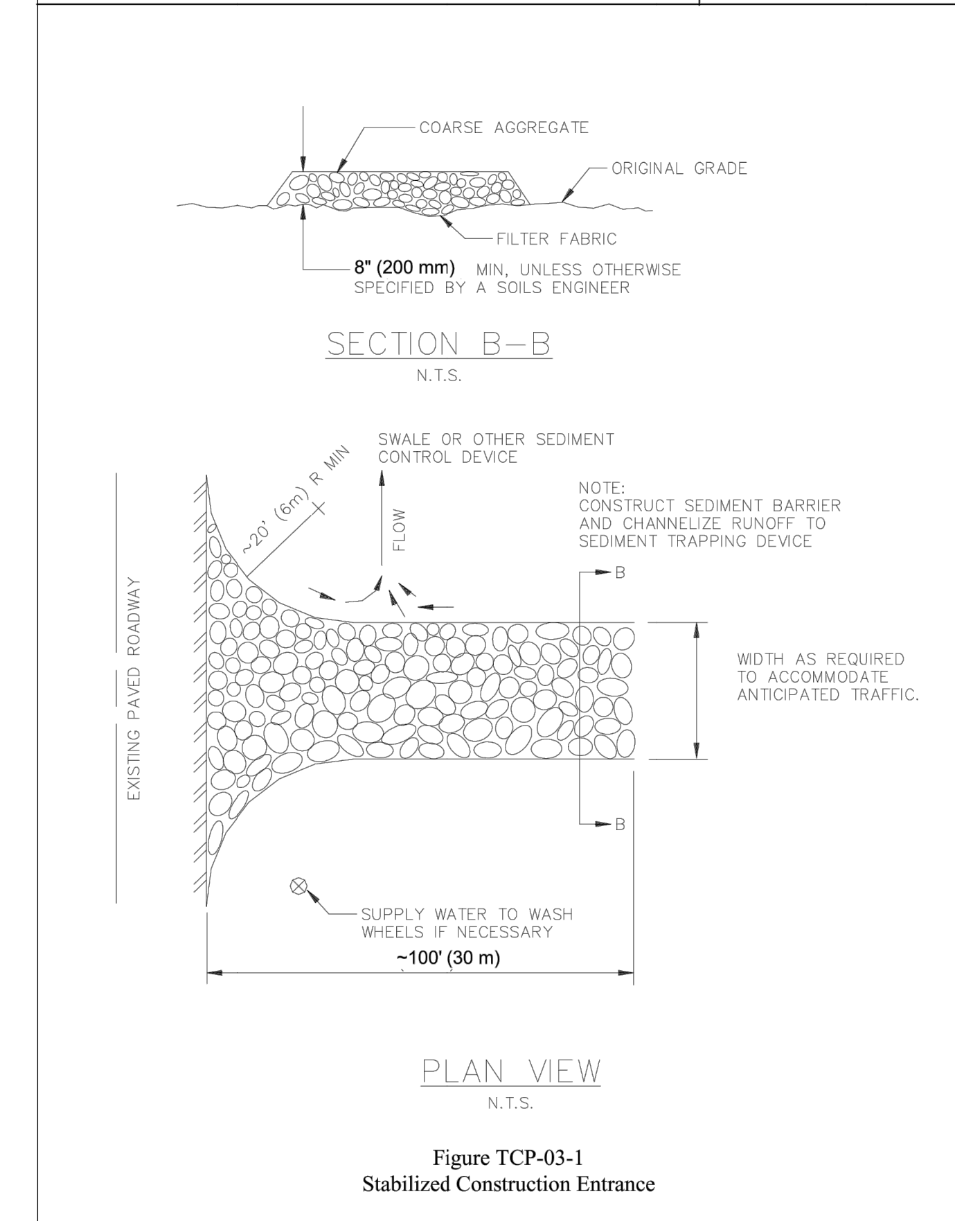
Figure TCP-03-1 Stabilized Construction Entrance
