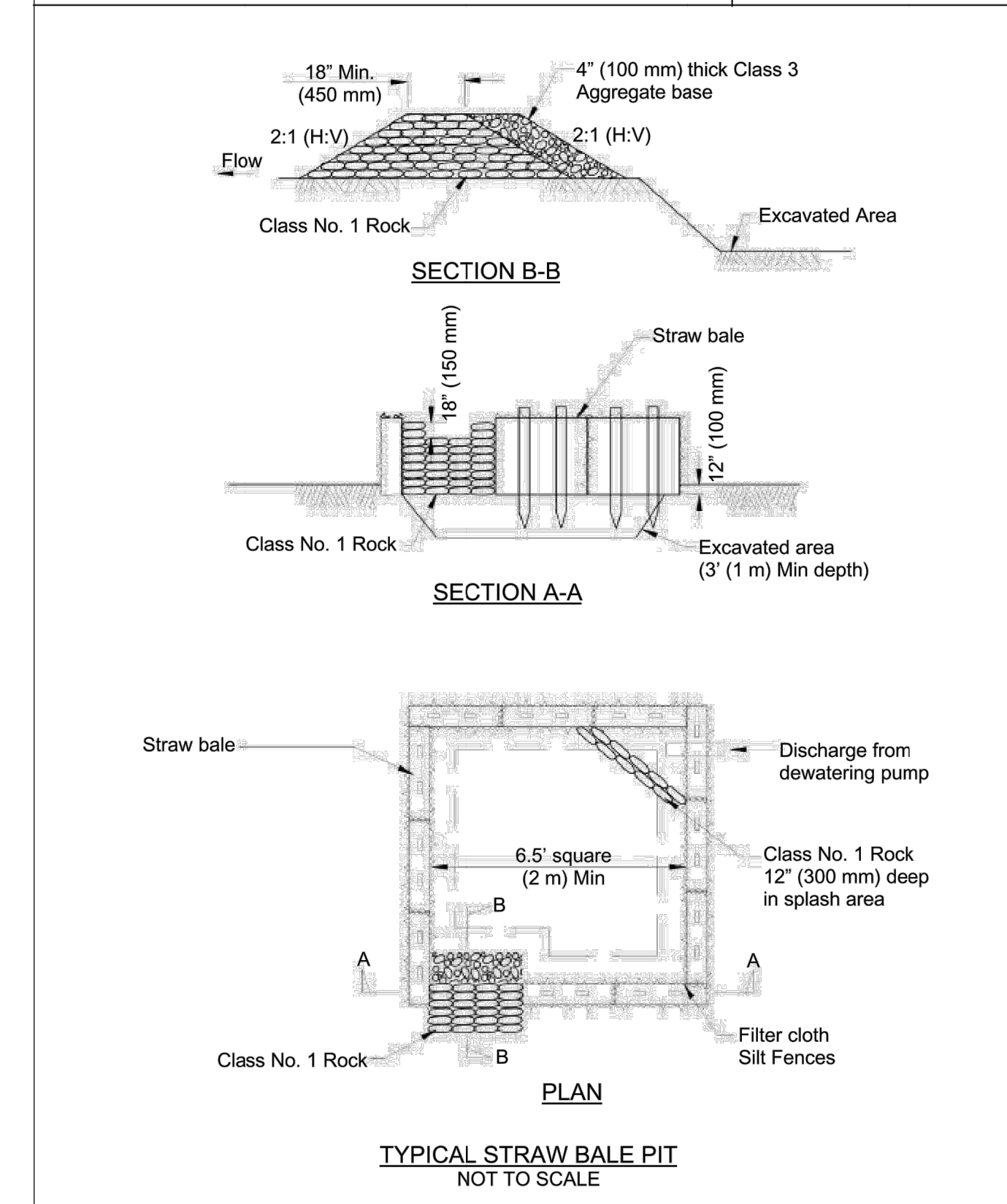
Figure CP-02-2 Typical Straw Bale Pit
