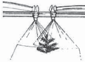
Figure 2b. Boom with overlapping nozzles spraying each row of trees.
